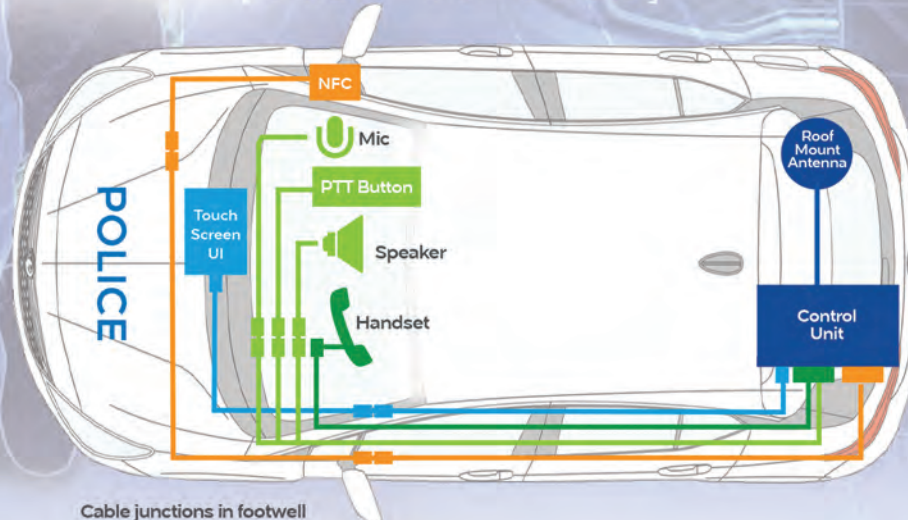
Cable junctions in footwell
